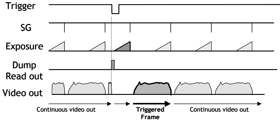
Fig. 10. Restart continuous trigger mode
